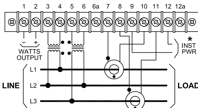
USING POTENTIAL AND CURRENT TRANSFORMERS
