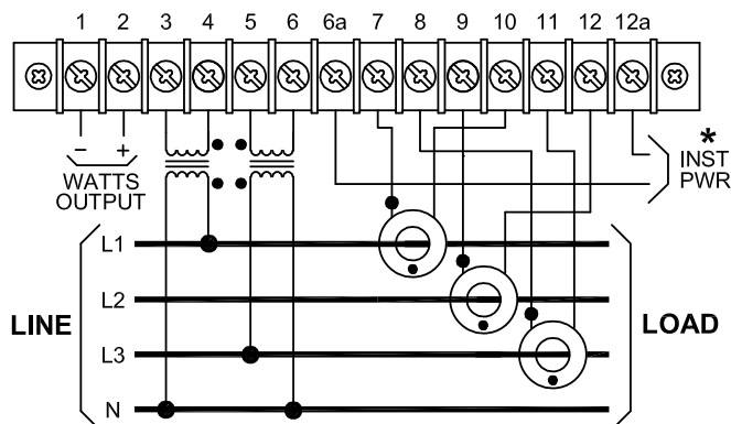
USING POTENTIAL AND CURRENT TRANSFORMERS
